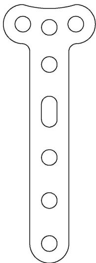
3.5mm Right Angle Part No. 001815 5 holes in shaft 3 holes in head
