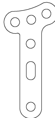
3.5mm Oblique Thick Part No. 001820 3 holes in shaft 3 holes in head
