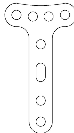
3.5mm Right Angle Part No. 001814 4 holes in shaft 4 holes in head
