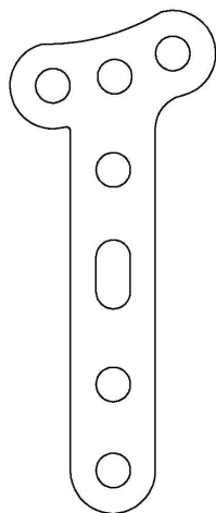
3.5mm Oblique Part No. 001818 4 holes in shaft 3 holes in head
