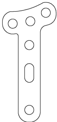
3.5mm Oblique Part No. 001817 3 holes in shaft 3 holes in head
