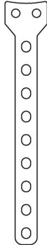
3.5mm T-Plate Part No. 000642 9 holes in shaft 2 holes in head
