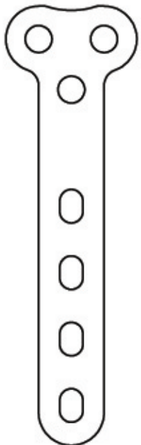
3.5mm Tibial Wedge Part No. 002314 4 holes in shaft 3 holes in head
