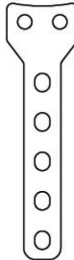
3.5mm T-Plate Part No. 002612 5 holes in shaft 2 holes in head
